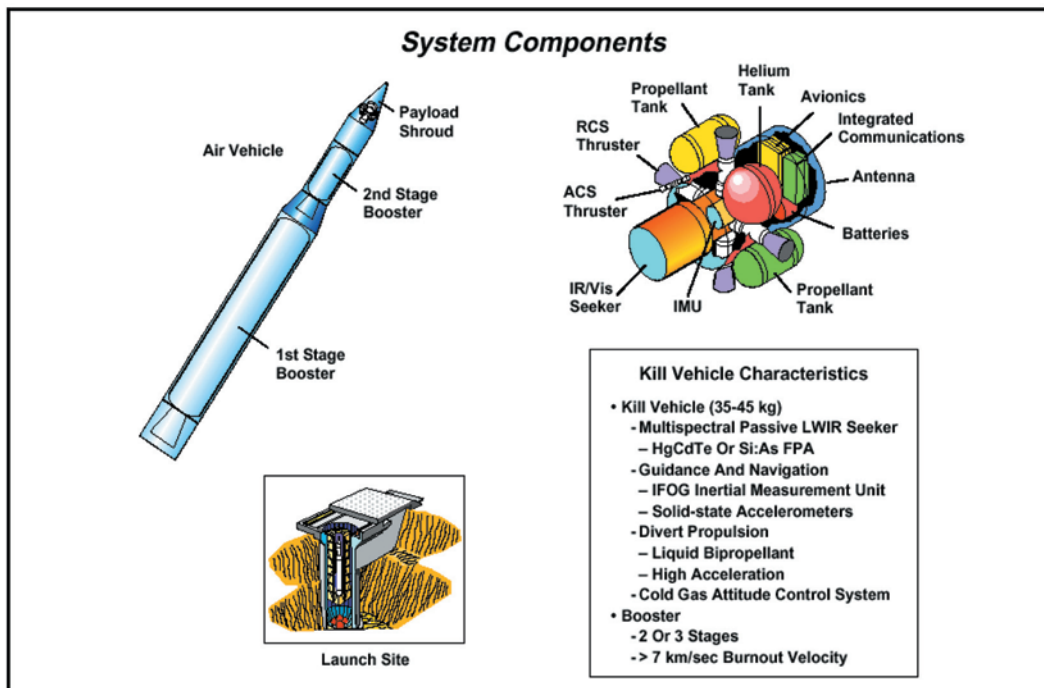
Figure 21.3: Ground-based interceptors. Source: BMDO 1997: 92, at: < http://www.acq.osd.mil/bmdo/bmdolink/html/bmdolink.html >.
