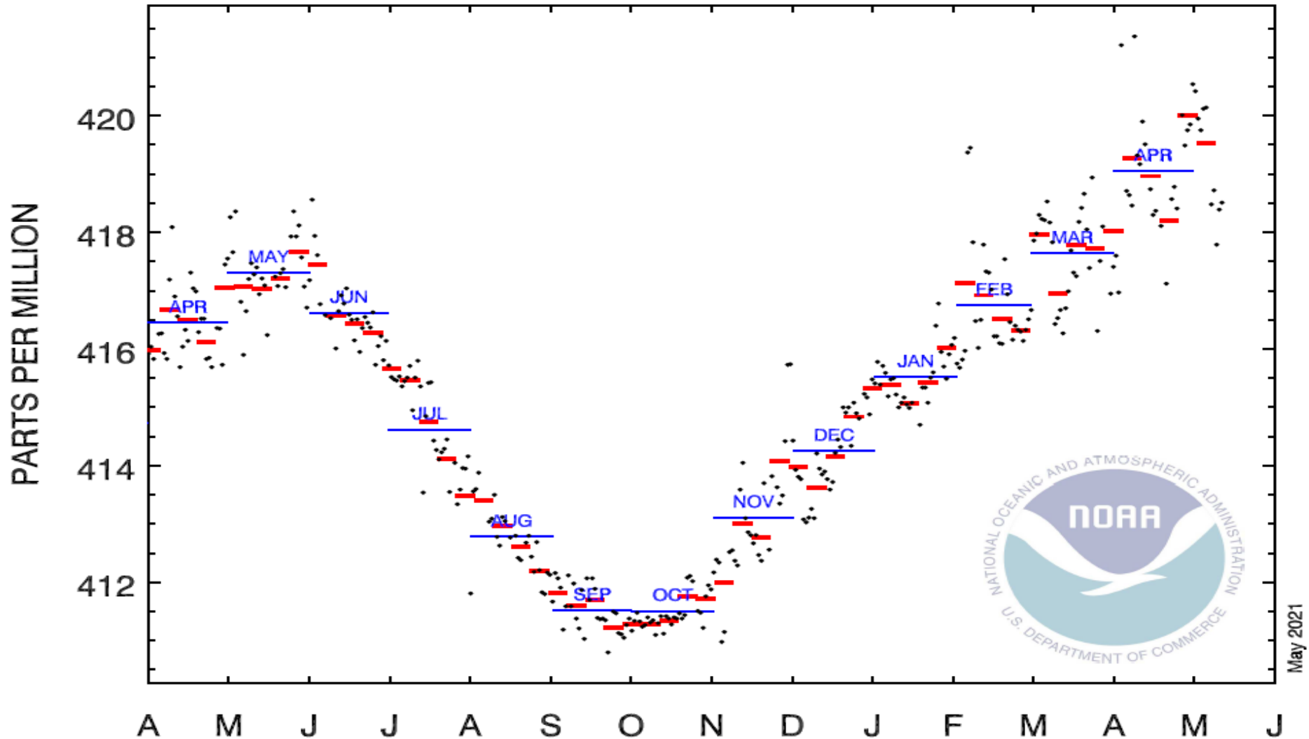
One year of CO 2 daily and weekly means at Mauna Loa
