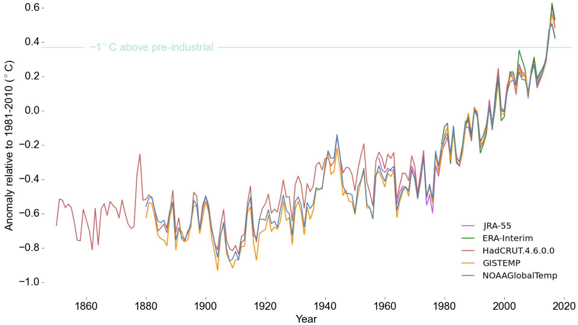
Global temperature anomaly 1850-2017 relative to 1981-2010
